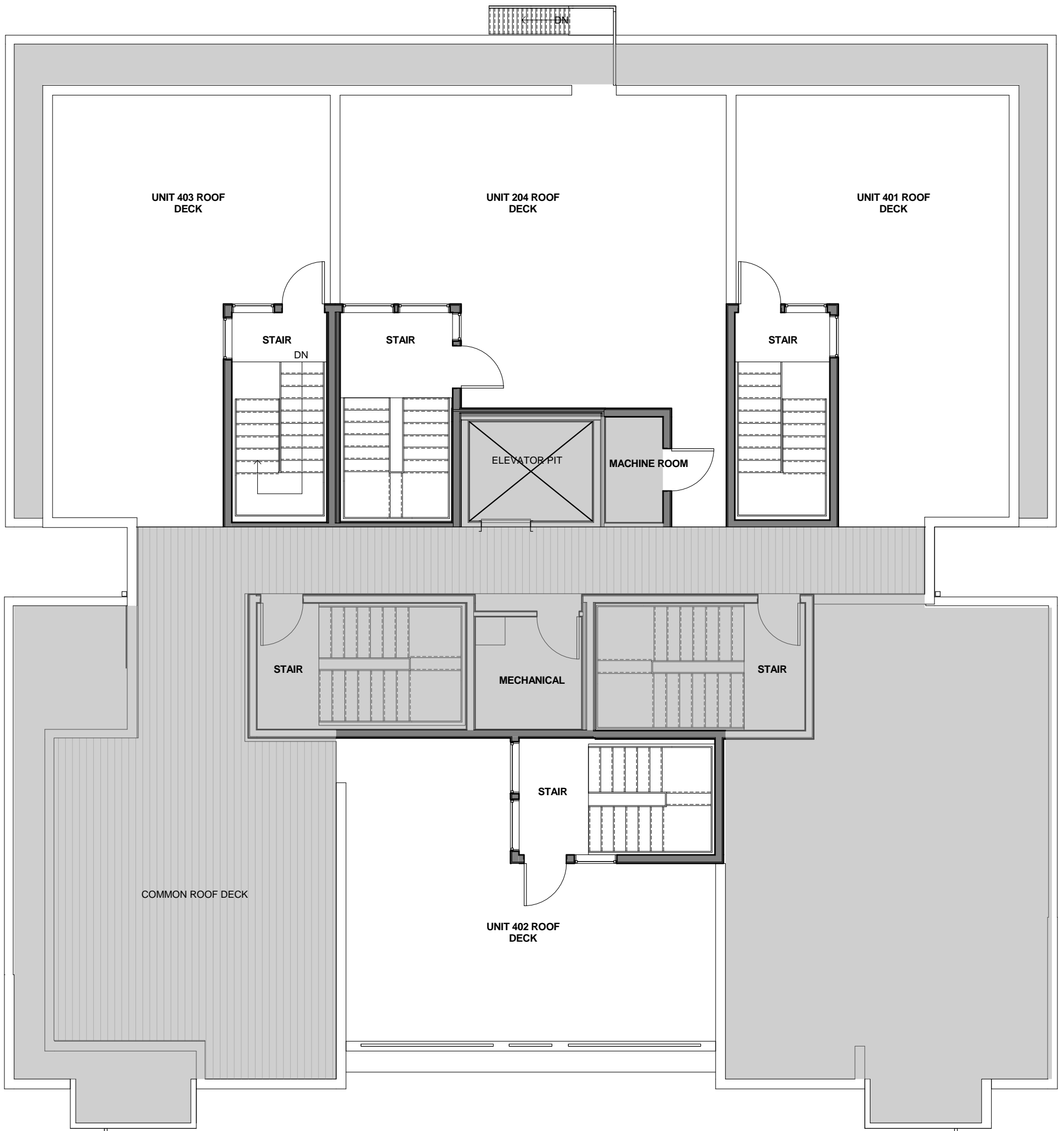
ROOF DECK PLAN
